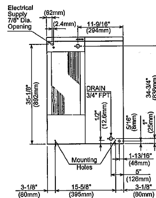
AIR-COOLED UNIT
