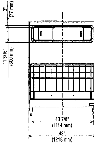
FRONT VIEW B-1150/1300SS
