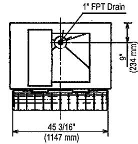
TOP VIEW B-1150/1300SS
